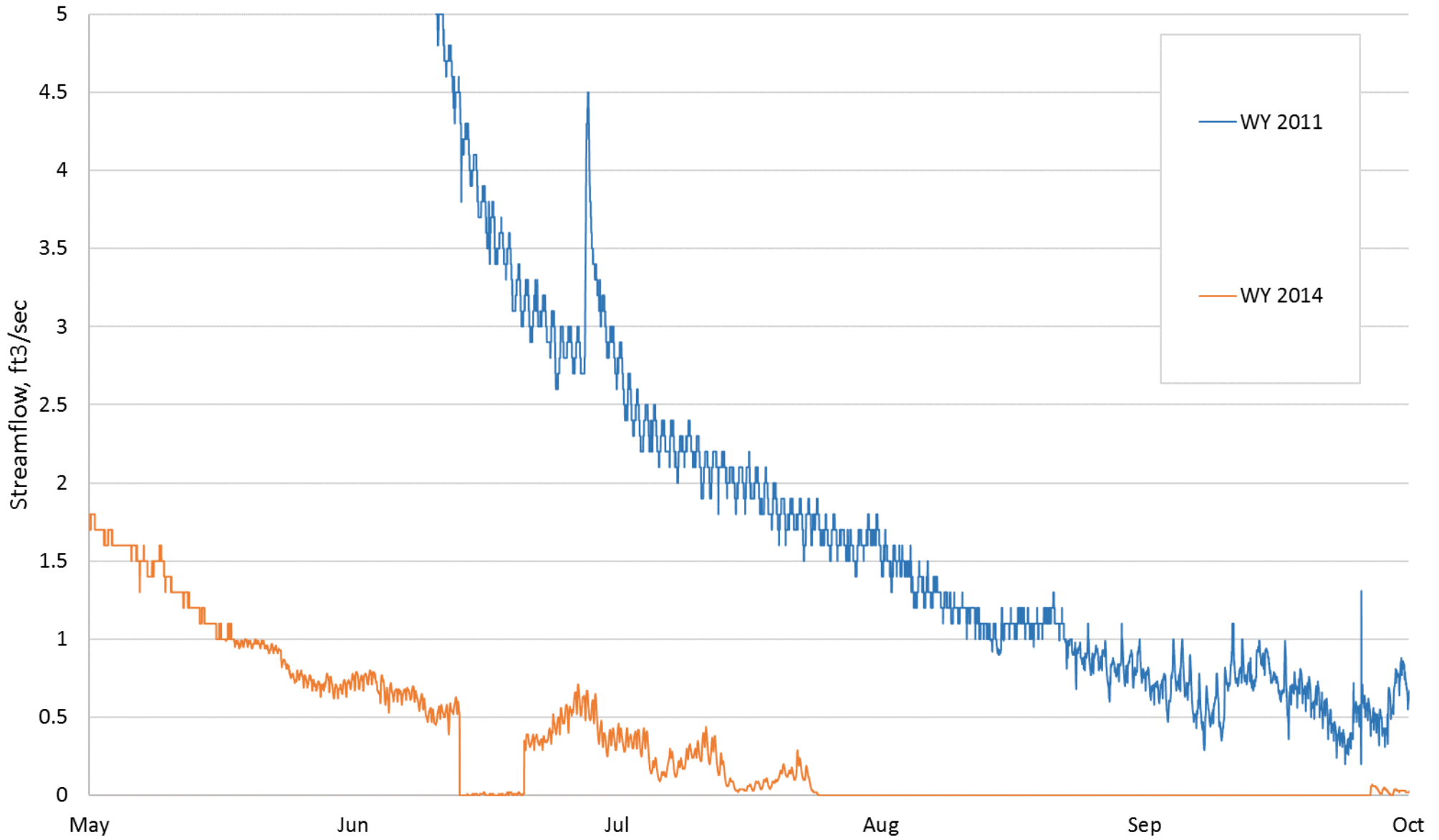
Mill Creek - Streamflow, WY 2011 & 2014
