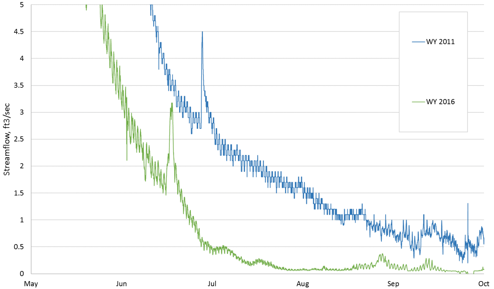
Mill Creek - Streamflow, WY 2011 & 2016
