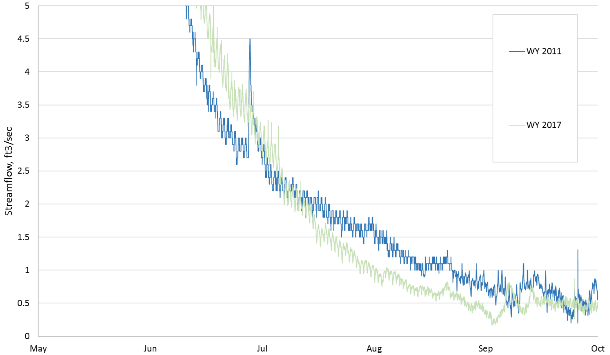
Mill Creek - Streamflow, WY 2011 & 2017
