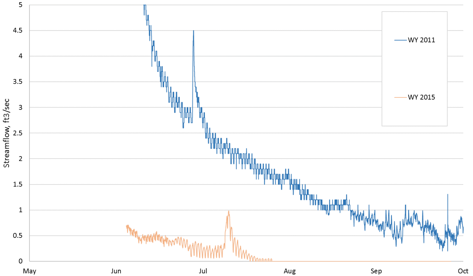
Mill Creek - Streamflow, WY 2011 & 2015
