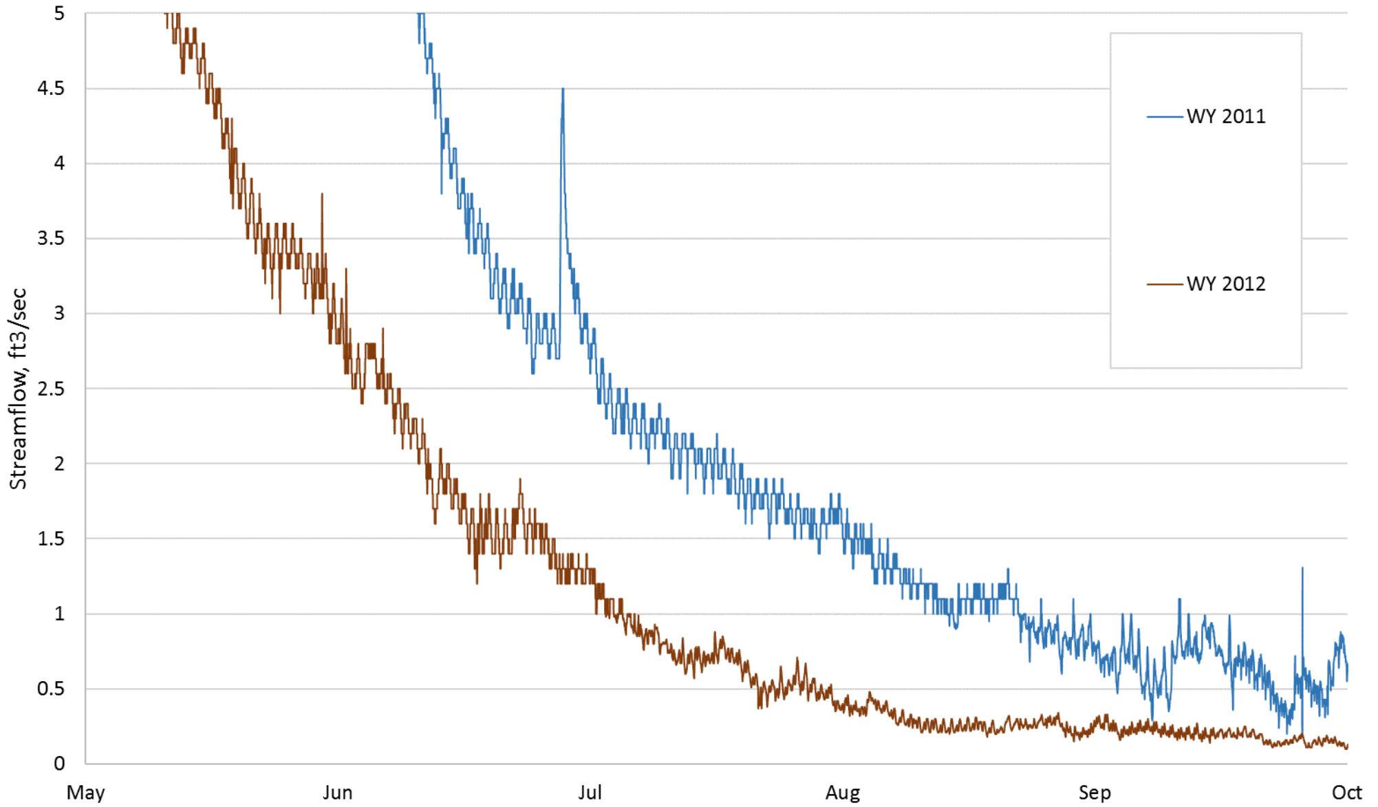
Mill Creek - Streamflow, WY 2011-2012
