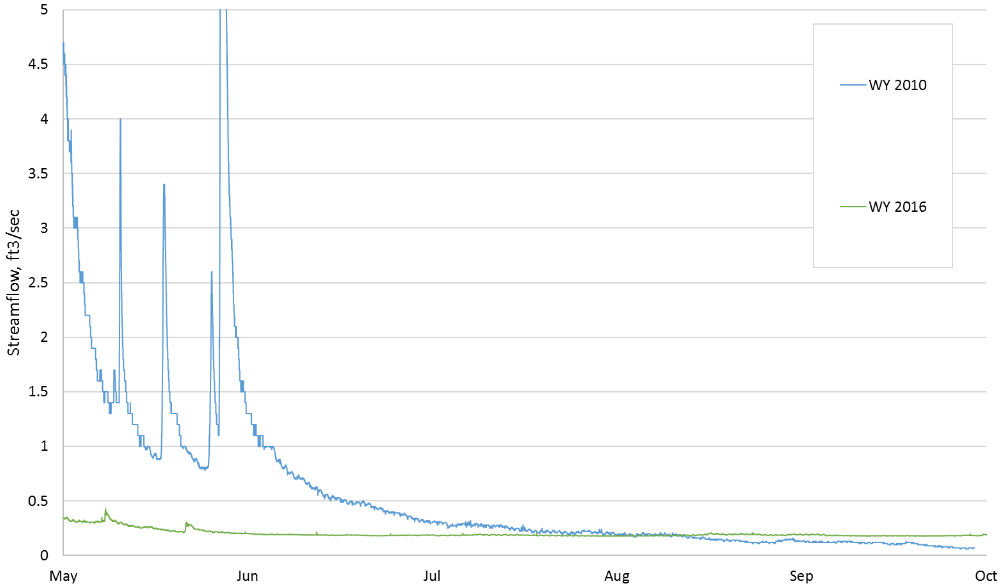
Mark West Creek - Streamflow, WY 2010 & 2016
