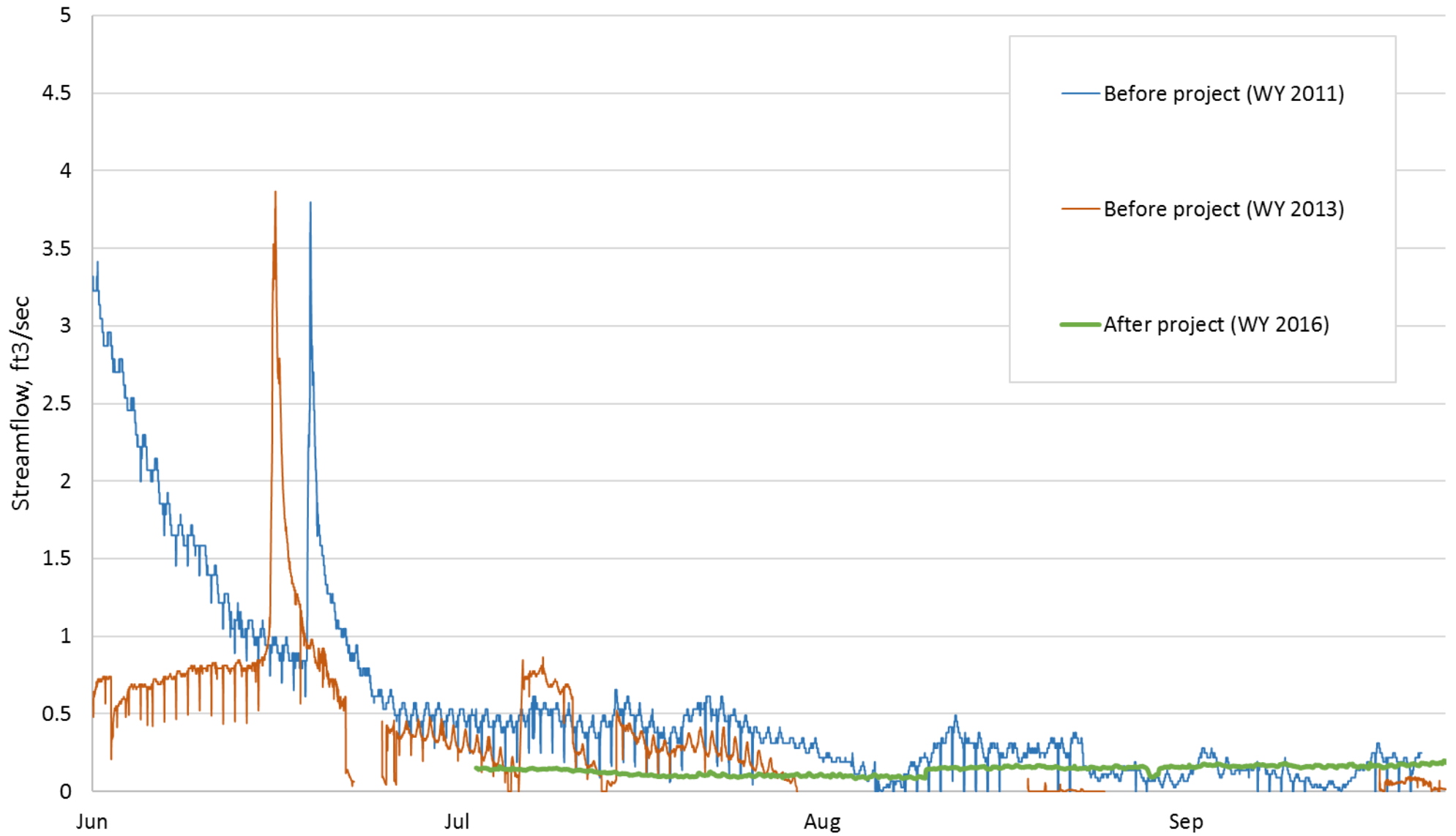
Dutch Bill Creek - Streamflow, before and after project
